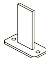
PIASTRA 130x60 2 FORI SP. 7 mm
